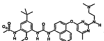
N-[5-tert-Butyl-3-(3-{4-[2-(2-dimethylamino-ethylamino)-6-methyl-pyrimidin-4-yloxy]-naphthalen-1-yl}-ureido)-2-methoxy-phenyl]-methanesulfonamide;
